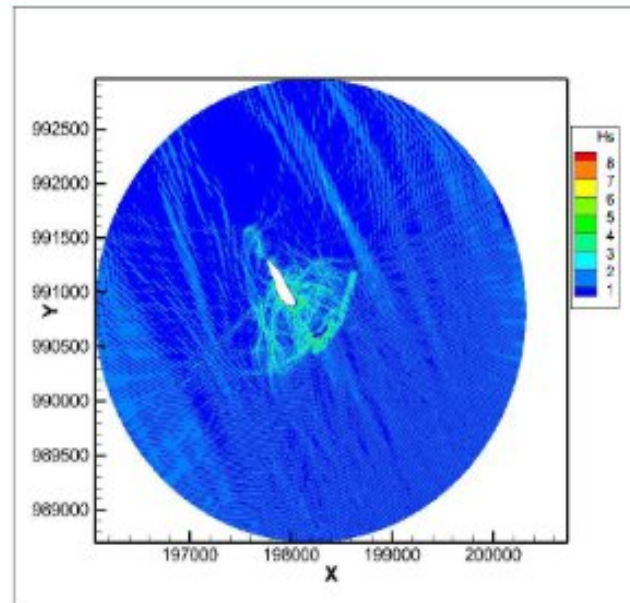
Figure 8 Wave height distribution for the wave approach angle from 135^\circ for Kariyachalli Island with Artificial reef
